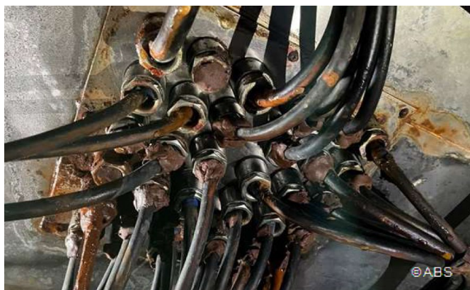
Water leaking through the Multi Cable Transit (MCT) in lobby
